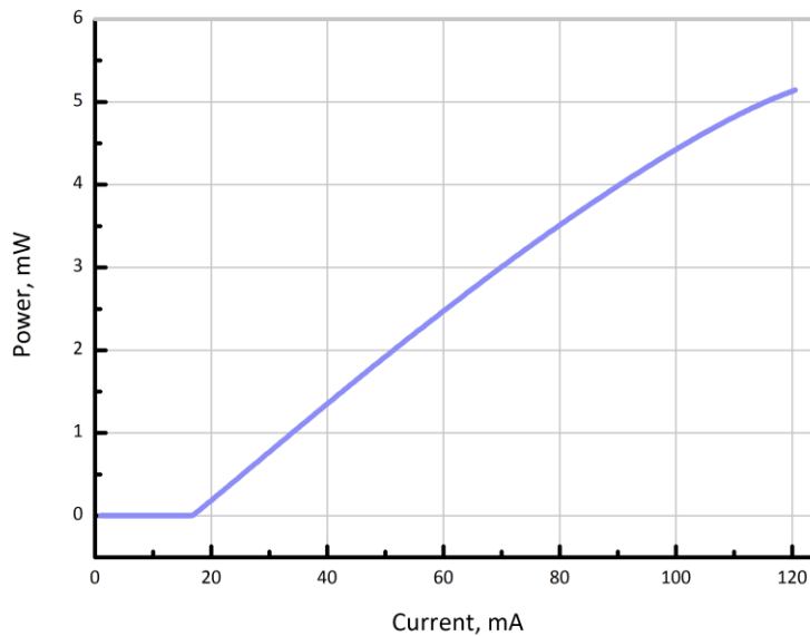
Power vs. Operating Current
